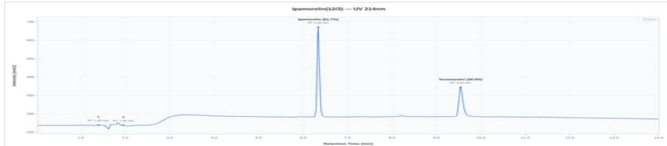
Tesamorelin / Ipamorelin 12/3 - TEIPF726: UV Chromatogram
