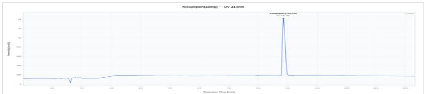
KISSPEPTIN 10mg - K102726SS: UV Chromatogram
